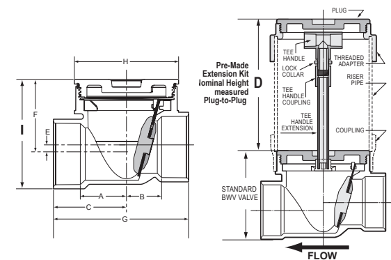
VALVE DIMENSIONS Table 1
